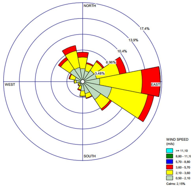
Fig. 22. Direction of incidence in the winds from jan/22 to dec/22
